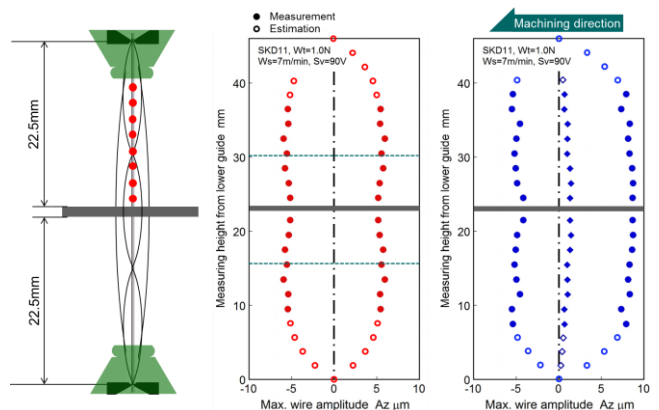
Fig. 4 Amplitude envelope of wire electrode
